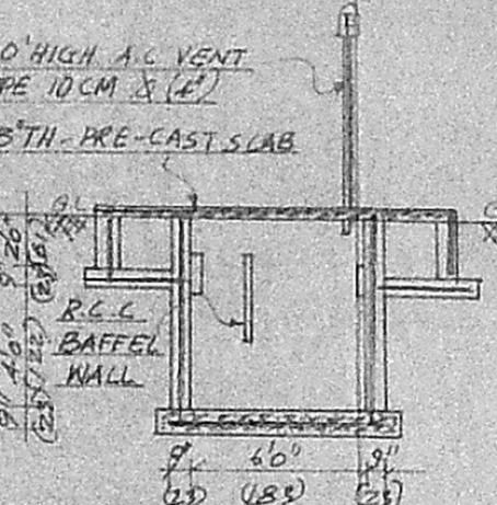
PLAN AND SECTION OF SEPTIC TANK.
